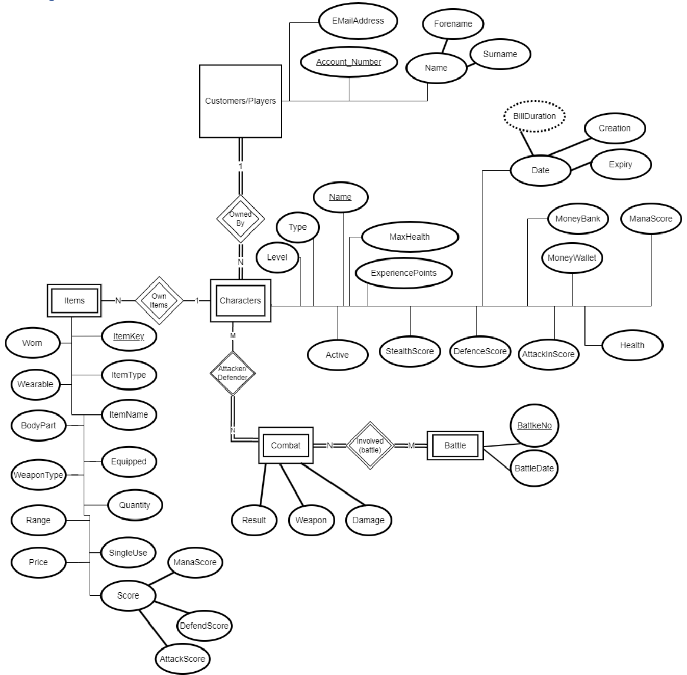
Overall ER diagram
